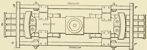
Fig. 12. Plan of Bolster and Spring Plank
